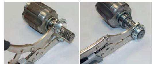
Clamps come down automatically when the joint opens. Ideal for saving the axle shaft without risking damage and having to replace it completely.
